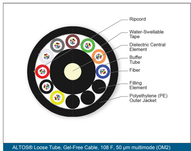
ALTOS® Loose Tube, Gel-Free Cable, 108 F, 50 µm multimode (OM2)
